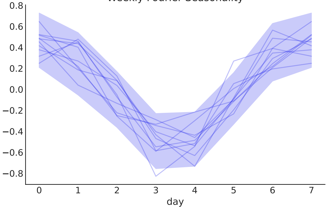
Weekly Fourier Seasonality
